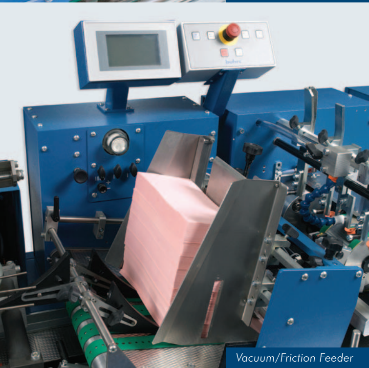
Pick & Place Feeder
